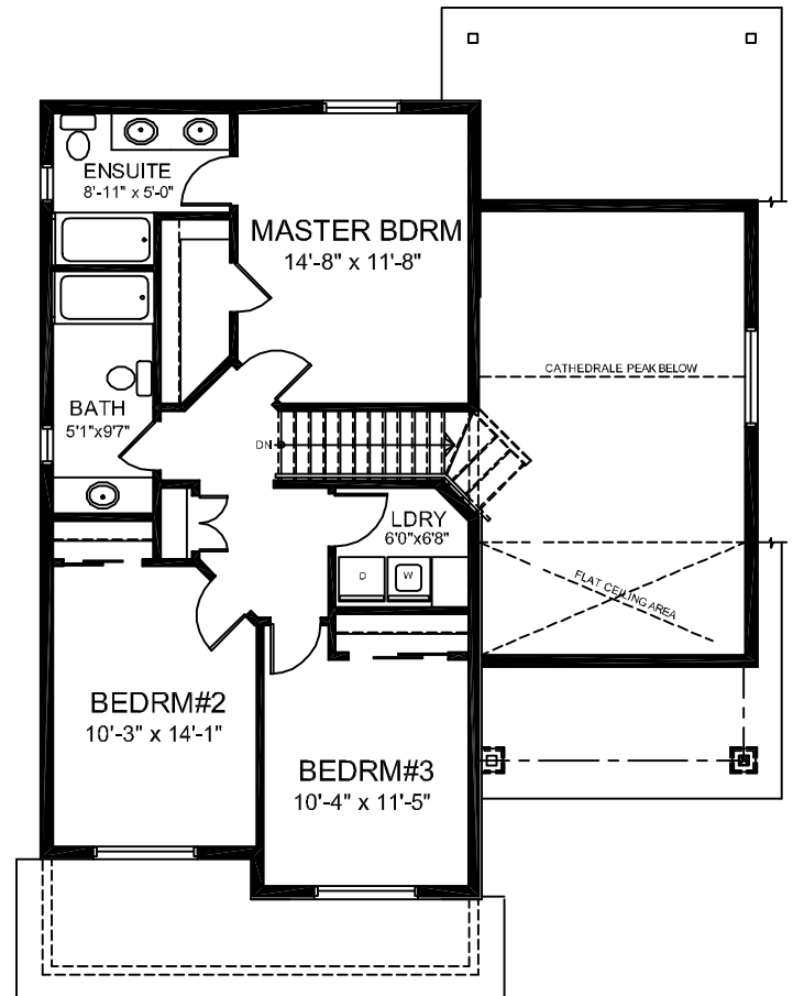
2nd STOREY FLOOR PLAN
